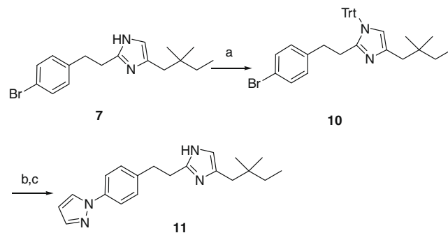
Scheme 2. Synthesis of 11 . Reagents and conditions: (a) TrtCl, TEA, CH 2 Cl 2 , 72%; (b) pyrazole, NaH, Cu, DMF; (c) TFA, 95% (two steps).
