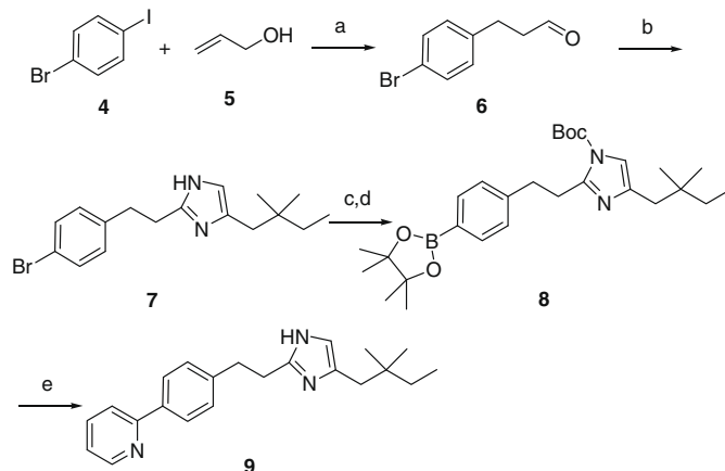
Scheme 1. Synthesis of 9 . Reagents and conditions: (a) Pd(OAc) 2 , Bu 4 NCl, NaHCO 3 , DMF, 40 °C, 85%; (b) A , NH 4 OAc, Cu(OAc) 2 in AcOH, 100 °C, 40 min, 45%; (c) Boc 2 O, TEA, DMAP in CH 2 Cl 2 , 1 h at rt, 80%; (d) bis(pinacolate)diboron, Pd(dppf), KOAc, DMF, 2 h, 85%; (e) 2-bromopyridine, Pd(dppf), Na 2 CO 3 (2 N), DMF, 85 °C, overnight, 72%.
